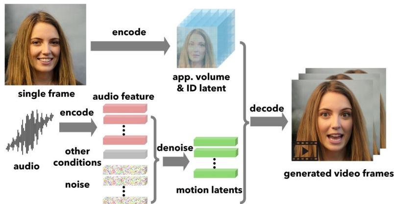
Test pipeline for audio to video generation
