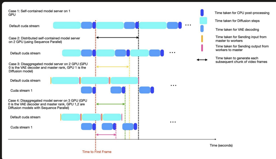
Figure: TalkingMachines runtime analysis, Character.AI, arXiv 2506.03099.
