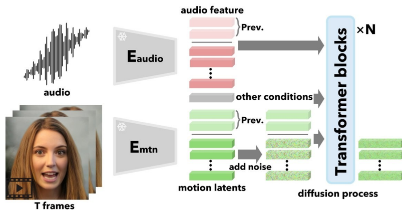
Training pipeline for motion latent diffusion
