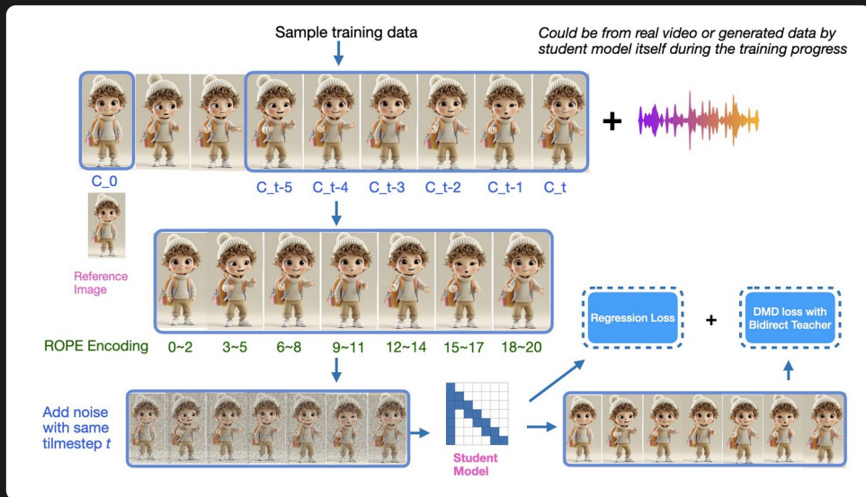
Figure: TalkingMachines, Character.AI, arXiv 2506.03099 (2025).
